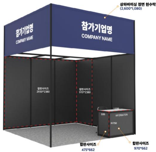
Perspective View
